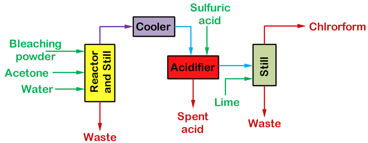
Figure: Manufacture of Chloroform from acetone and bleaching powder
